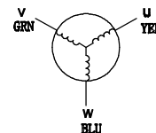
Motor phases
