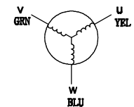
Motor phases
