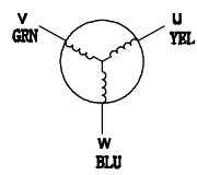
Motor phases
