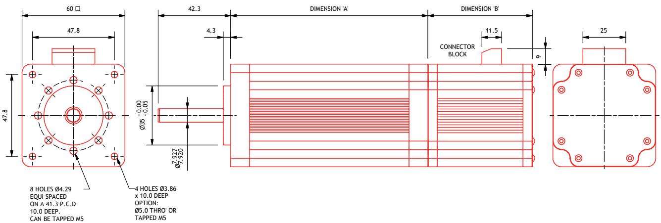
PBL60IE with standard flange/mount and shaft
