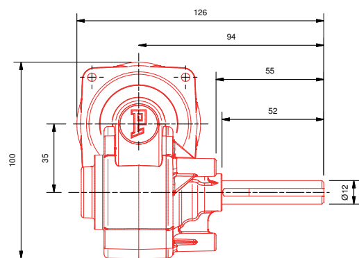
Parvalux M3P fixing option
