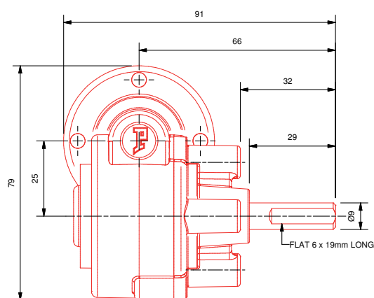
Parvalux S3P fixing option
