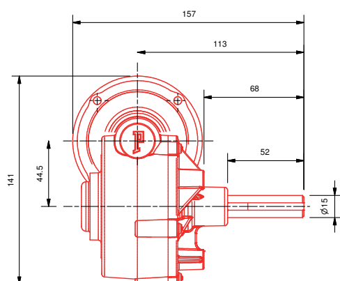
Parvalux L3P fixing option
