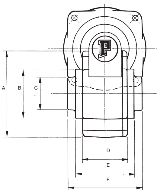
NOMINAL AS CAST DIMENSIONS ± 0.13mm
