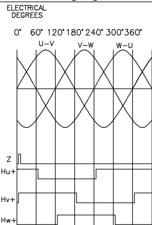
Timing diagram
