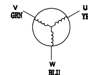
MOTOR CONNECTIONS
